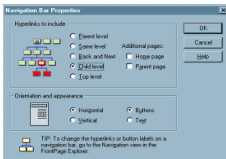
Gambar 3. Navigation Bar
