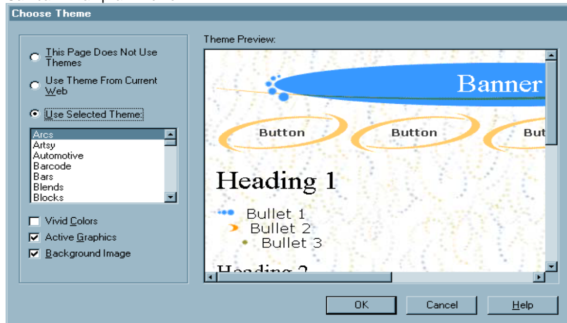
Gambar 2. Tampilan Theme
